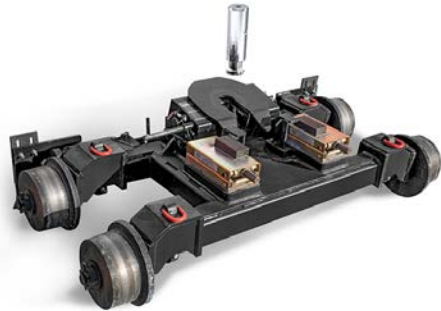
NON-WELD INTERFACE 4-WHEEL DOLLY
